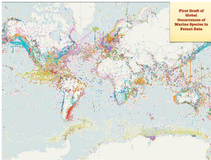
Figure 22. First draft of global occurrences of marine species in patent data (Oldham, et al., 2013).
